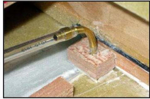
(above) Vent/overflow tube position inside the wing tank bay.
