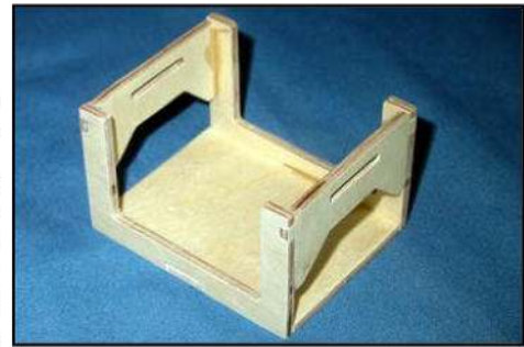
(above) Assemble hopper tank mount from the milled plywood.
