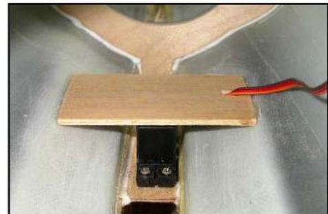
(above) Rudder servo mount is installed for you at the factory. (below) Servo installed with balsa protection glued in position.
