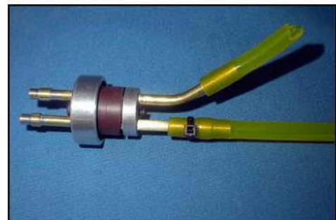
(above) Detail view of the fuel tank cap assembly, with the short lengths of 4mm I.D tube soldered on to act as 'barbs' and prevent the tubing sliding off.
