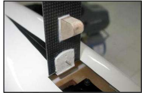
(above) Nosegear door hinge glued and screwed in position. (below) Nose door should have 1mm gap all round.
