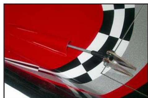
(above) Secure rudder & stab servo extensions to fuselage. Cover rudder servo plate with aluminium tape for heat protection. (below) Rudder linkage fairing.
