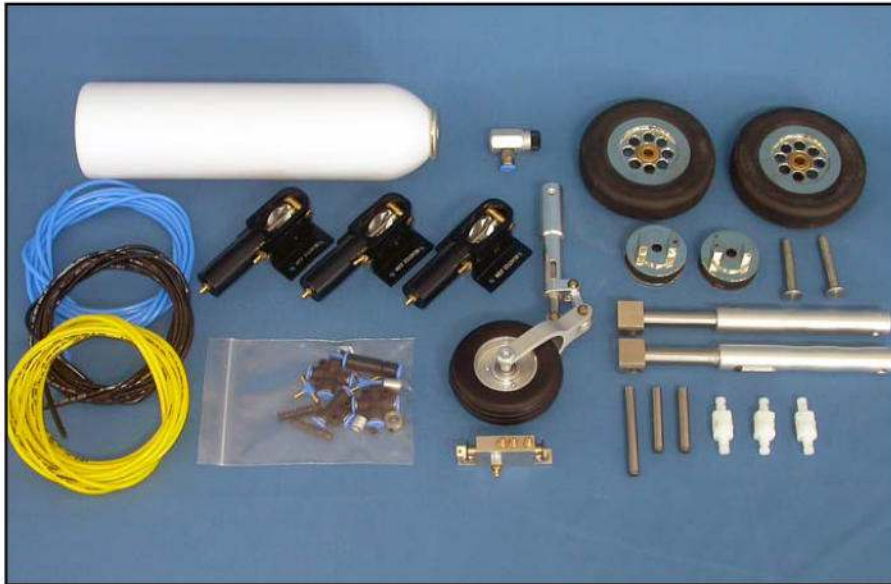
(above) CARF Landing Gear set for Flash (Optional)
