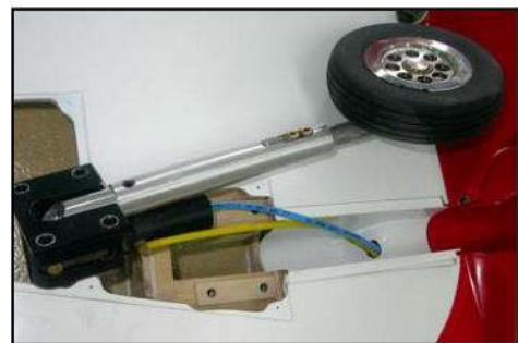
(below) Fibreglass leg covers trimmed and trial installed in wing for final adjustment. You can also see the ply packers used to adjust height of wheels in wheel-wells.
