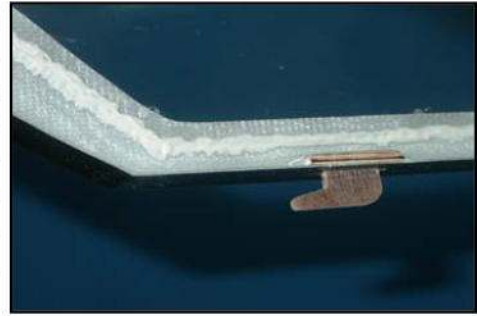
(above) Trap the inside edges of the clear canopy into the frame with a small bead of slow epoxy all around. Note also the phenolic canopy hooks seen here.
