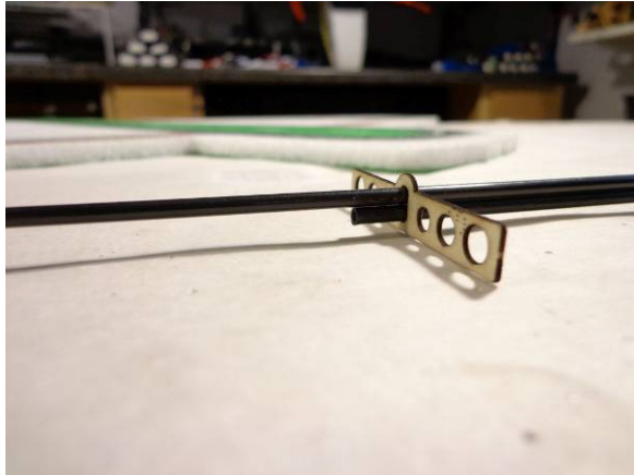
Close up of how the spars stack up inside the slot of the inner rib. No Glue
