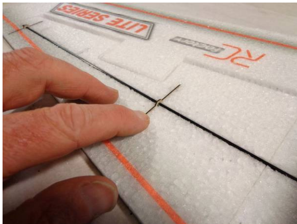
Make sure that the rib slots you cut and the precut spar slots are deep enough to allow everything to sit flush as shown above
