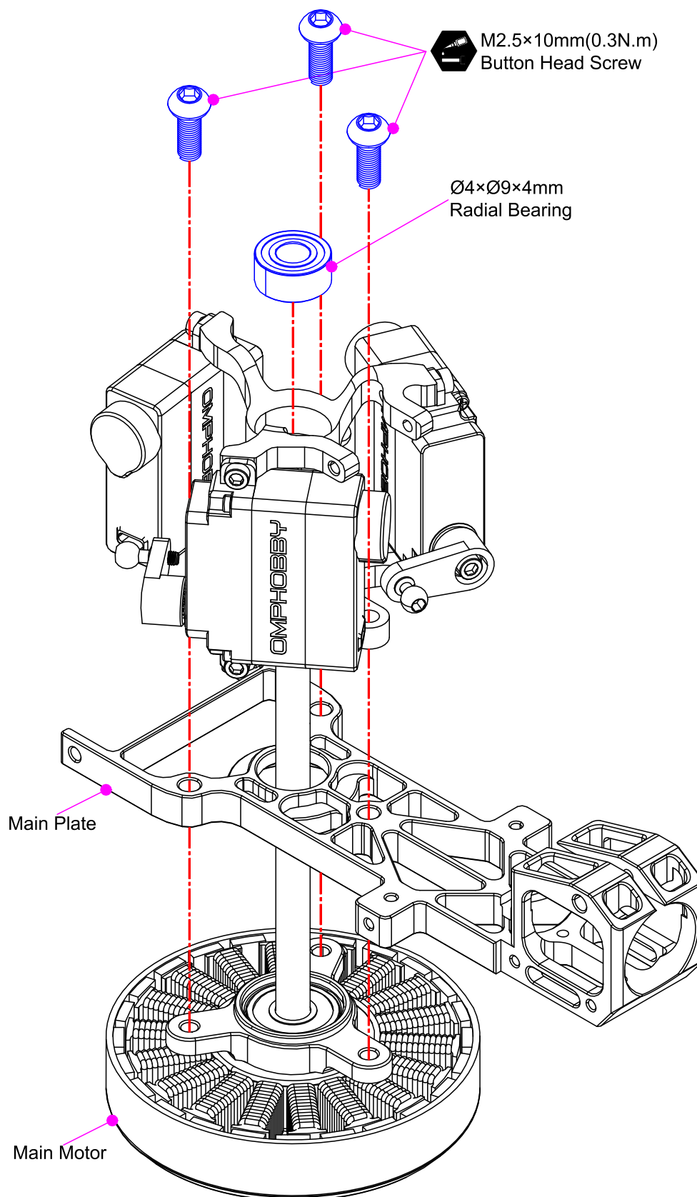
Button Head Screw (M2.5×10mm)x3
