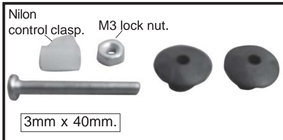
Control horn of elevator.
