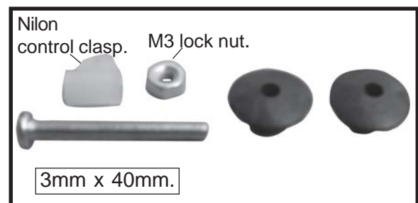
Control horn of Rudder.
