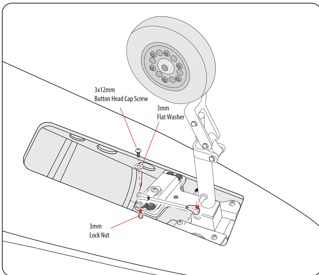
Bottom view
